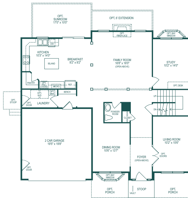
FIRST FLOOR PLAN SULLIVAN
