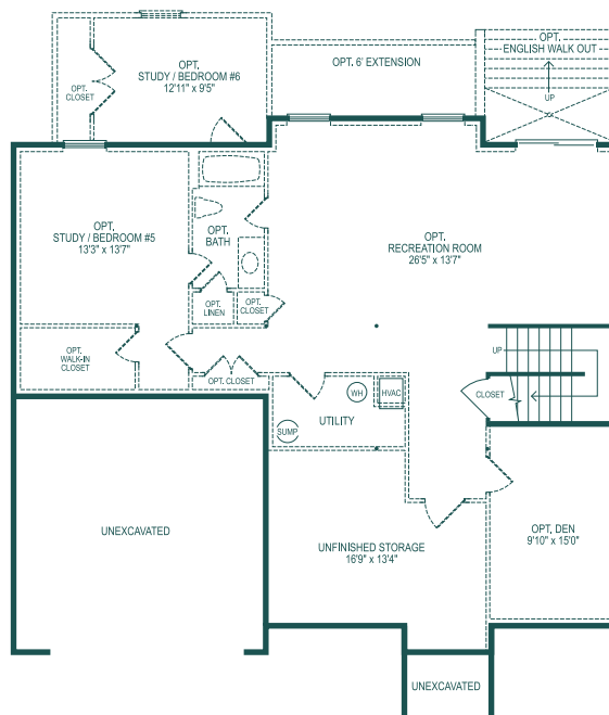
BASEMENT FLOOR PLAN SULLIVAN
